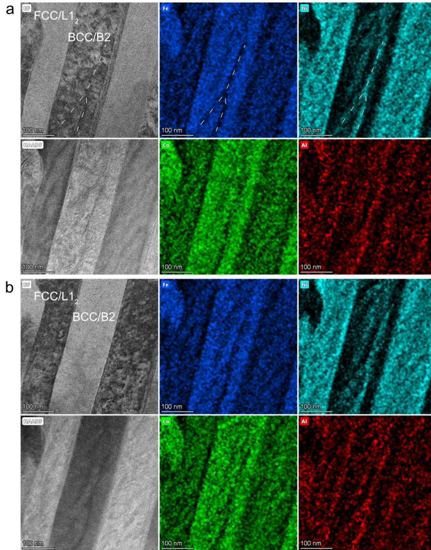
Figure S1. BF and HAADF STEM images and corresponding Fe (blue), Co (green), Ni (cyan) and Al (red) EDXS elemental maps. In (a), the BCC column is at a crystallographic zone axis orientation, while in (b) the FCC column is at a crystallographic zone axis orientation. A 3° tilt was applied along the horizontal direction between the two orientations. Note the upside-down 'Y'-shaped dashed line, which marks the Ni-Al-rich inclusion at which the magnetic field lines are interrupted in Fig. 4(b), suggesting that such regions are either very weakly magnetic or non-magnetic.
