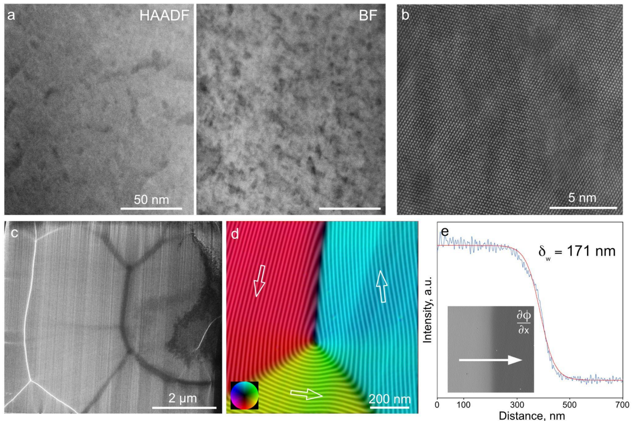
Figure 1. Microstructural and magnetic imaging of the CRSA sample. (a) HAADF STEM and BF STEM images show local variations in chemical composition and diffraction contrast originating from Ni/Al-rich precipitates. The HAADF detector inner semi-angle was 69 mrad for the HAADF STEM image. (b) Atomic-resolution HAADF STEM image. (c) Fresnel defocus image showing black and white contrast at the positions of magnetic domain walls recorded in magnetic-field-free conditions at a defocus of 1 mm. (d) Magnetic induction map of a flux closure region measured using off-axis electron holography. The contour spacing is \pi radians. Arrows and colors indicate the projected in-plane magnetic field directions. (e) Magnetic domain wall width measurement using the (inset) phase shift differential across the 180^\circ wall shown in (d). The magnetic domain wall width ( \delta_w ) is determined to be 171 \pm 5 nm.
