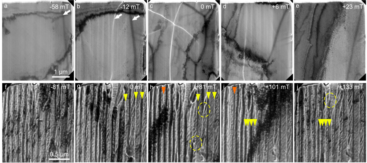
Figure. 5: Magnetization switching processes. Fresnel defocus images showing (a-e) nucleation-type magnetization reversal in the CRSA sample and (f-j) pinning-type magnetization reversal in the CRSA600 sample. The effective in-plane field was applied in the horizontal direction and is indicated in the images. The defocus value is 500 \mu\text{m} . In (a) and (b), arrows mark the positions of magnetic domain walls. In (g) and (h), yellow and orange arrowheads mark the positions of magnetic domain walls that switch in (h) and (i), respectively. Dashed ovals mark the positions of Bloch caps in domain walls. Note the presence of diffraction contrast (in particular, wide bands of dark contrast associated with slight bending of the sample) in addition to magnetic domain wall contrast.
