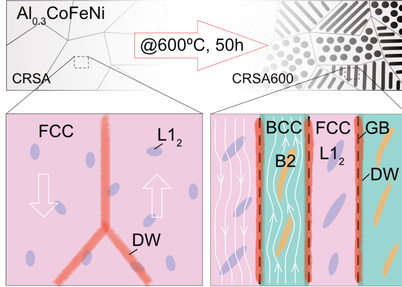
Figure 6. Schematic diagram showing the structural and magnetic characteristics of the \text{Al}_{0.3}\text{CoFeNi} complex concentrated alloy samples. Magnetic domain walls (DW) form and move freely within the \text{FCC} + \text{L}_{12} alloy, while they are pinned at heterophase boundaries between the \text{FCC} + \text{L}_{12} and \text{BCC} + \text{B}_2 regions. In the \text{BCC} + \text{B}_2 region, magnetic field lines (white, arrowed) embrace weakly magnetic \text{B}_2 precipitates.
