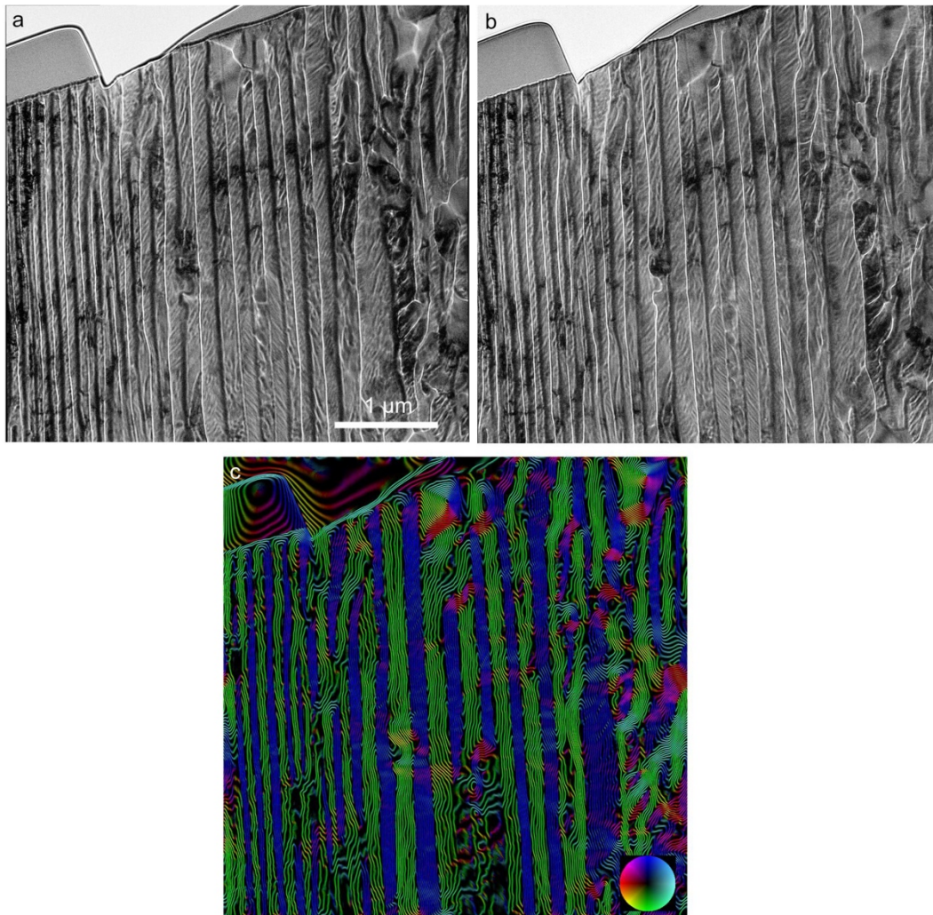
Figure S2. Large-field-of-view (a) underfocus and (b) overfocus Fresnel images and corresponding (c) magnetic induction map recovered from (a, b) using the transport-of-intensity equation. The image defocus value is 0.25 mm. The contour spacing is 2\pi/6 radians.
