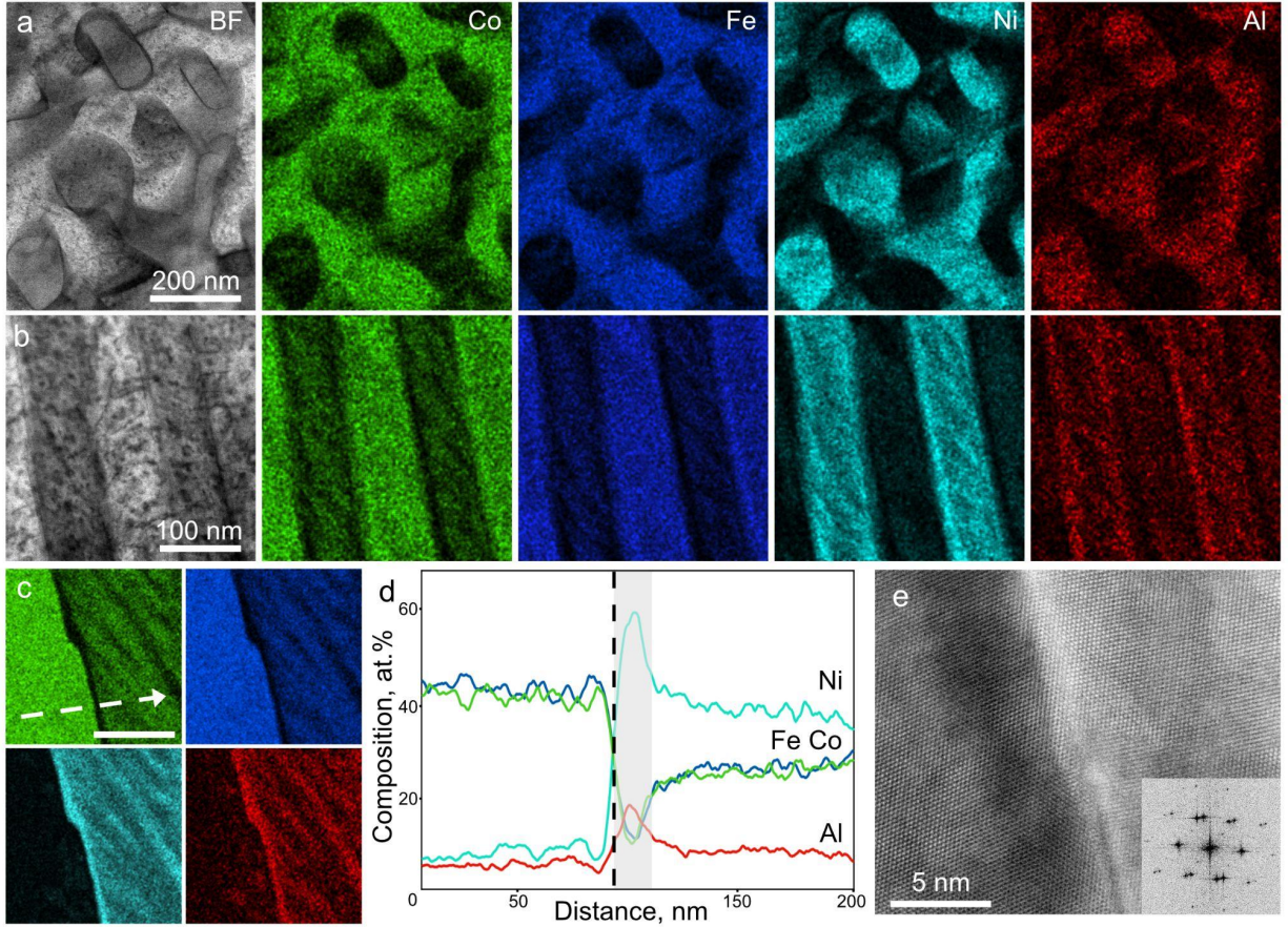
Figure 3. Microstructure and chemical composition of the lamellar structure in the CRSA600 sample. (a, b) BF STEM images and corresponding Co, Fe, Ni and Al EDXS maps recorded from (a) region II and (b) region I. (c) Higher magnification EDXS maps of the interface between the BCC and FCC columns. The scale bar is 100 nm. (d) Elemental distribution across the interface (marked by a dashed line) extracted from the EDXS spectrum images shown in (c). The shaded area is rich in Ni, Al and depleted in Fe, Co. (e) High-resolution HAADF STEM image of the interface. The inset shows a digital diffractogram of the crystallographic relationship between the FCC and BCC phases.
