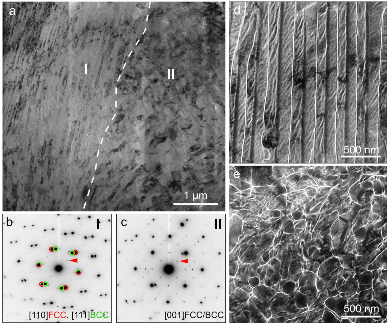
Figure 2. Microstructural and magnetic imaging of the CRSA600 sample. (a) BF TEM image showing the lamellar structure viewed from the side (I) and parallel to their long directions (II). (b, c) SAED patterns recorded from regions I and II. Red arrows mark superlattice reflections that are associated with \text{L1}_2 and B2 ordering. (d, e) Fresnel defocus images recorded at a defocus of 0.25\ \text{mm} defocus from regions I and II, respectively.
