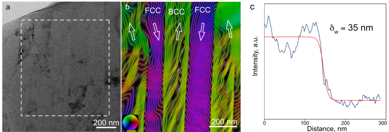
Figure 4. Magnetic domains in the CRSA600 sample. (a) Amplitude image of the FCC and BCC columns. (b) Magnetic induction map recorded using off-axis electron holography from the marked region in (a), showing alternating magnetic field directions in the domains. Colors and arrows indicate the projected in-plane magnetic field directions. Note the regions with lower densities of magnetic field lines in the BCC columns. The upside-down ‘Y’-shaped region (marked by dashed white lines) is confirmed to be Ni-Al-rich from EDXS measurements (Fig. S1 in the Supplementary Information). (c) Line scan obtained from the phase differential (not shown) used to measure the magnetic domain wall width \delta_w as 35 \pm 3 nm.
